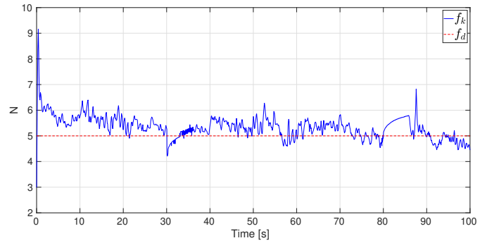
Fig. 14. Grasping force f_k and desired force f_d .
