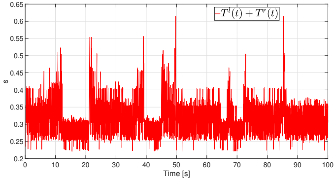
Fig. 10. Time-delay in the communication channel T^l + T^r .
