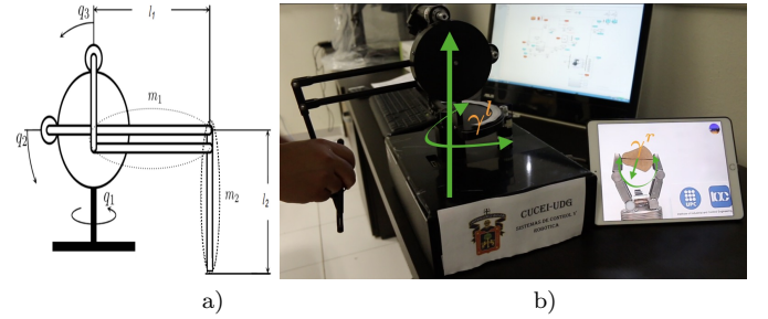
Fig. 2. a) PHANTOM Premium 1.5 High Force haptic device diagram, and, b) tested at local station located in Guadalajara, Mexico.
