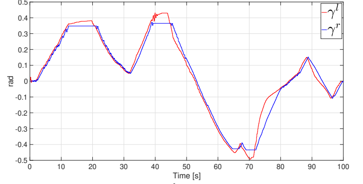
Fig. 6. Local orientation \gamma^l and remote object orientation \gamma^r .
