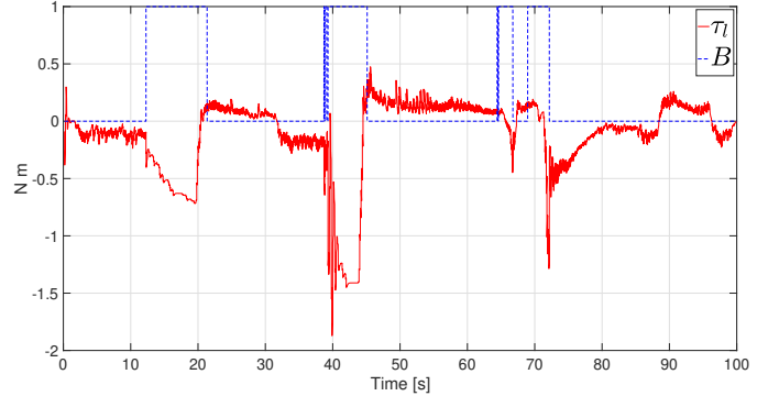
Fig. 7. Local torque \tau^l and the signal B indicating valid ( B = 0 ) and non valid ( B = 1 ) movements.
