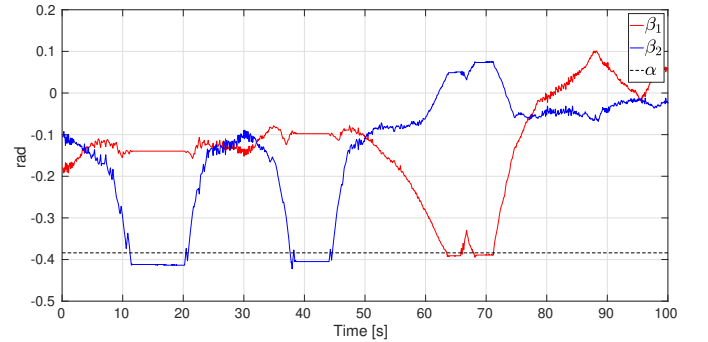
Fig. 8. Angles \beta_1 and \beta_2 , and the friction cone \alpha .
