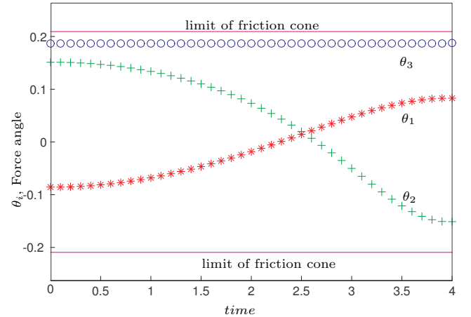
Fig. 10. Variation of the direction of \mathbf{f}_i (angle between the normal direction and \mathbf{f}_i ).
