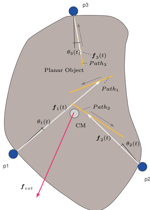
Fig. 11. Physical object, Path 1 , Path 2 and Path 3 , and forces \mathbf{f}_1 , \mathbf{f}_2 and \mathbf{f}_3 during the state transition.
