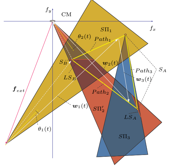
Fig. 7. GWL for S_A and S_B , including the initial forces in S_A , the final forces in S_B , and the paths Path_i for the three wrenches \mathbf{w}_i .
