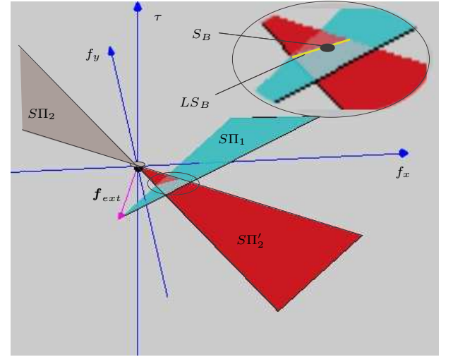
Fig. 5. GWL for S_B , the enlargement shows LS_B .
