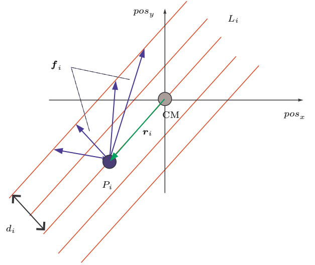
Fig. 2. Lines L_i of constant torque \tau_i due to forces \mathbf{f}_i applied at P_i .
