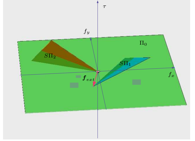
Fig. 4. \mathbf{f}_{ext} and two friction cones SII_1 and SII_2 .
