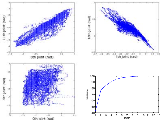
Fig. 1. Top-left: Positive correlation between proximal phalanges; Top-right: Negative correlation between the index and the ring abductions/adductions; Bottom-left: No correlation between the thumb base and the medium phalanx of the index; Bottom-right: Total variance covered as a function of the number of PMDs used. Reproduced from [15].
