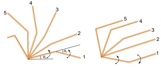
Fig. 3. Left: Motion of the 2 DOF planar robot along the first PMD that defines a positive coupling between the two joint angles \theta_1 and \theta_2 , i.e. both joints move in the positive (counterclockwise) sense. Right: Motion along the second PMD that defines a negative coupling, i.e. \theta_1 moves counterclockwise while \theta_2 moves clockwise.
