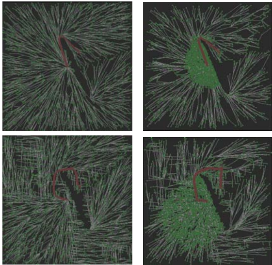
Fig. 7. RRT* optimizing distance (top): plain solution and solution using path bias and node filtering; RRT* optimizing the proposed cost (bottom): plain solution and solution using path bias and node filtering;
