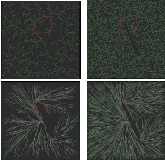
Fig. 4. RRT (top) and RRT* (bottom) for different number of samples.
