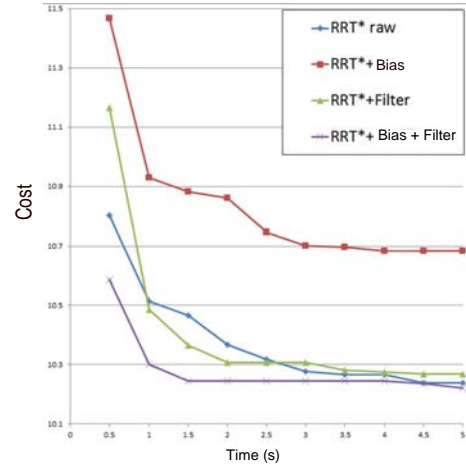
Fig. 6. Cost decrease as a function of time (in seconds) resulting from the average of 5 executions per planner.
